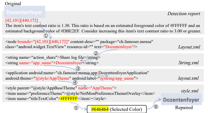
Figure 7: Example of attribute-to-repair localization for text contrast.
