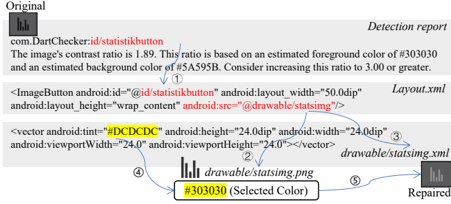
Figure 8: Example of attribute-to-repair localization for image contrast.
