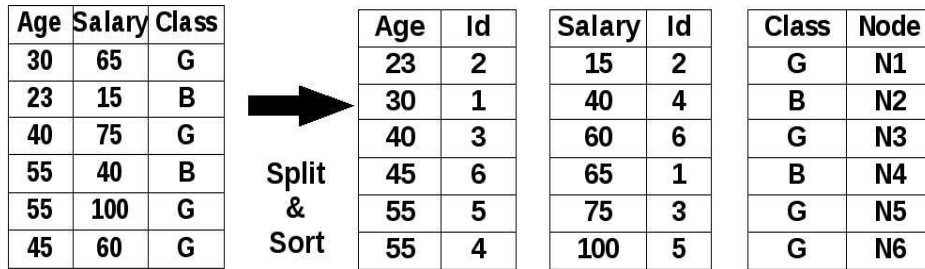
Figure 8 Representing the data in the form of sorted attribute lists and a class list.
