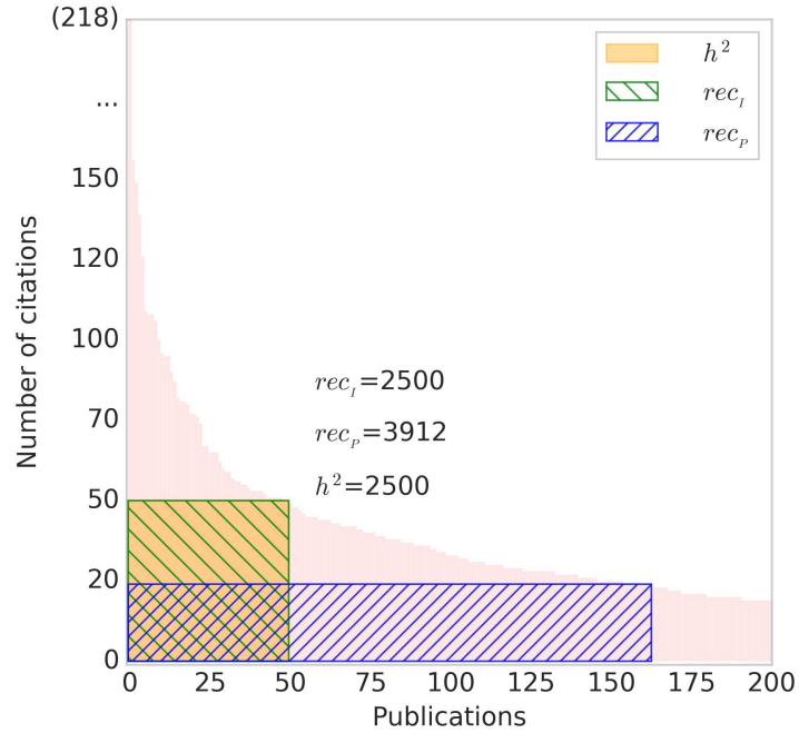
Figure 3: Example for class C2 of a Google Scholar author for which: rec_P \succ rec_I \approx h^2 .
