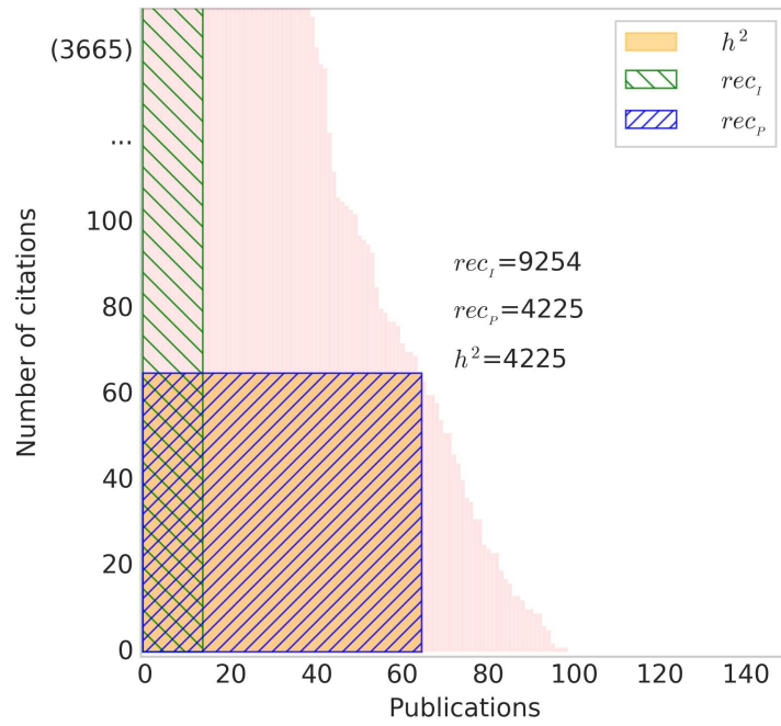
Figure 5: Example for class C1 of one of the two Nobel prize winners for which: rec_i \succ rec_p \approx h^2 , Greider, Physiology/Medicine, 2009.
