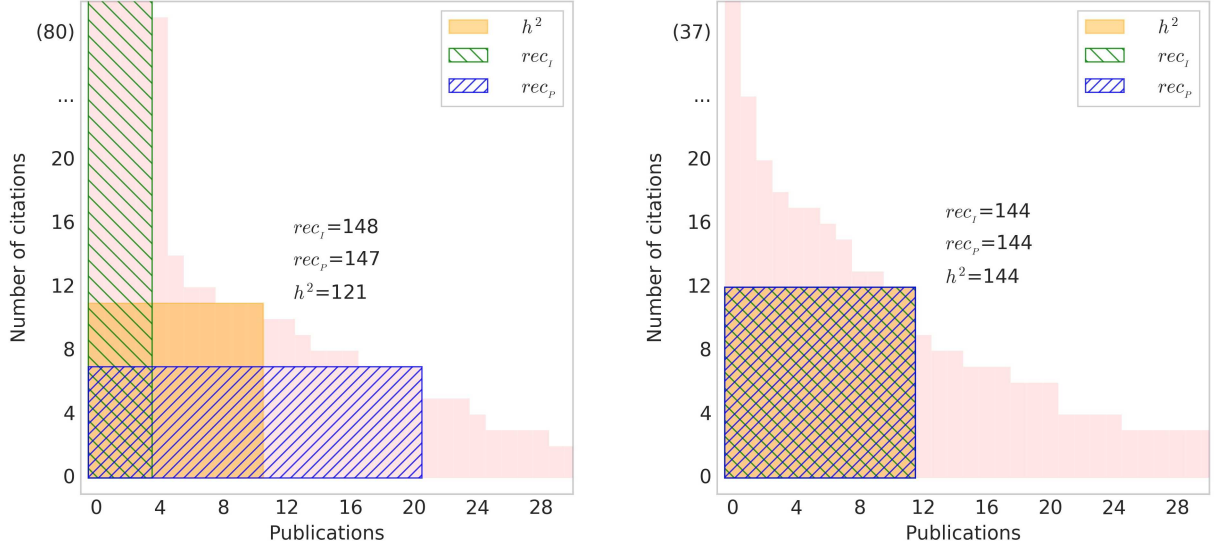
Figure 4: Examples for class C3 of Google Scholar authors for which: rec_I \approx rec_P > h^2 (left), rec_I \approx rec_P \approx h^2 (right).
