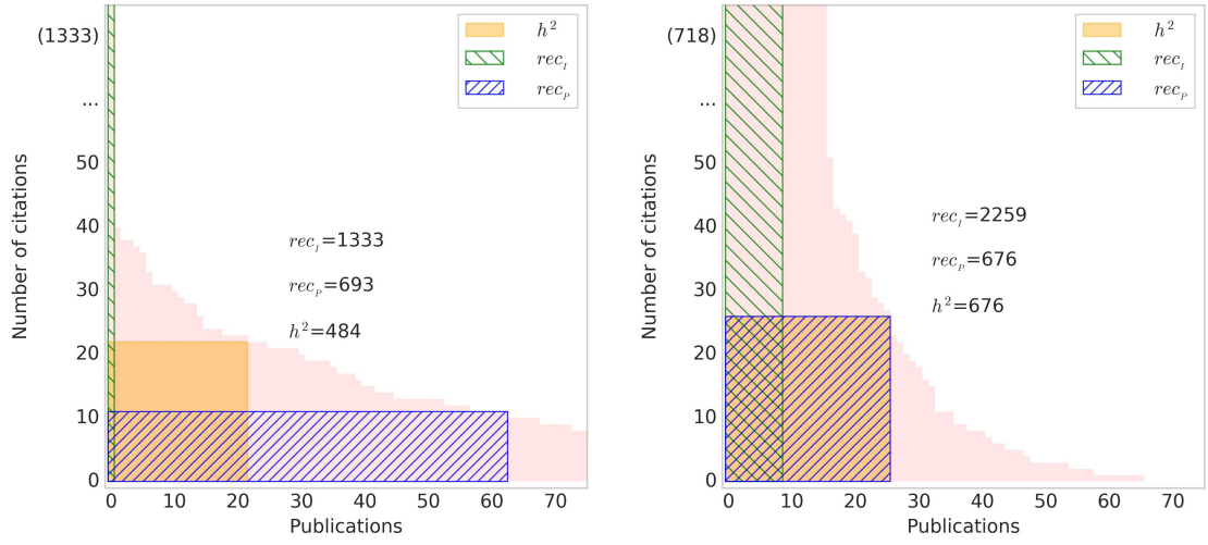
Figure 2: Examples for class C1 of Google Scholar authors for which: rec_I \succ rec_P \succ h^2 (left), rec_I \succ rec_P \approx h^2 (right).
