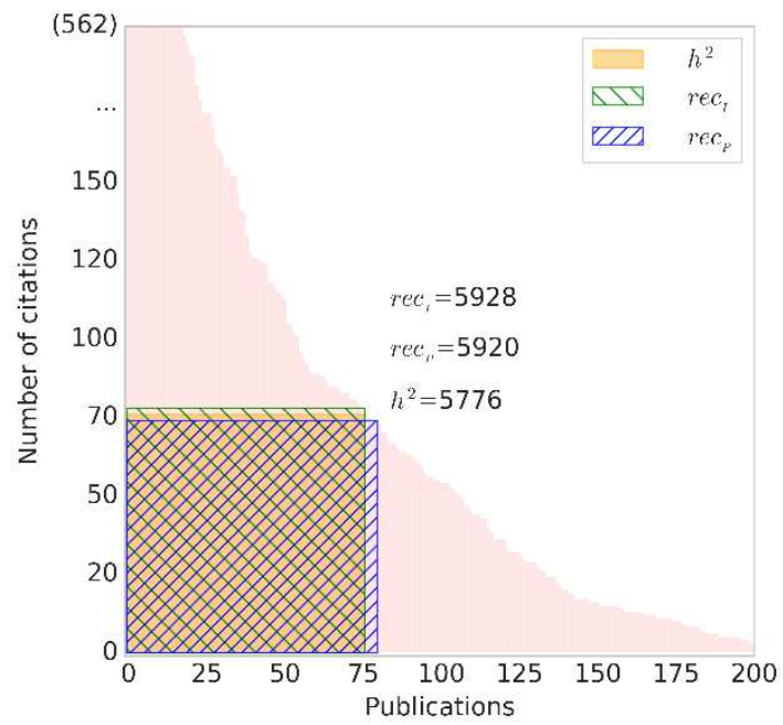
Figure 7: Example for class C3 of a Nobel prize winner for which: rec_I \approx rec_P \approx h^2 , Gurdon, Physiology/Medicine, 2012.
