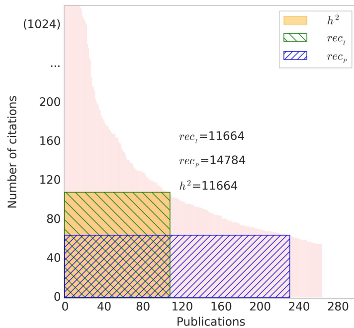
Figure 6: Example for class C2 of one of the two Nobel prize winners for which: rec_p \succ rec_i \approx h^2 , Schrock, Chemistry, 2005.
