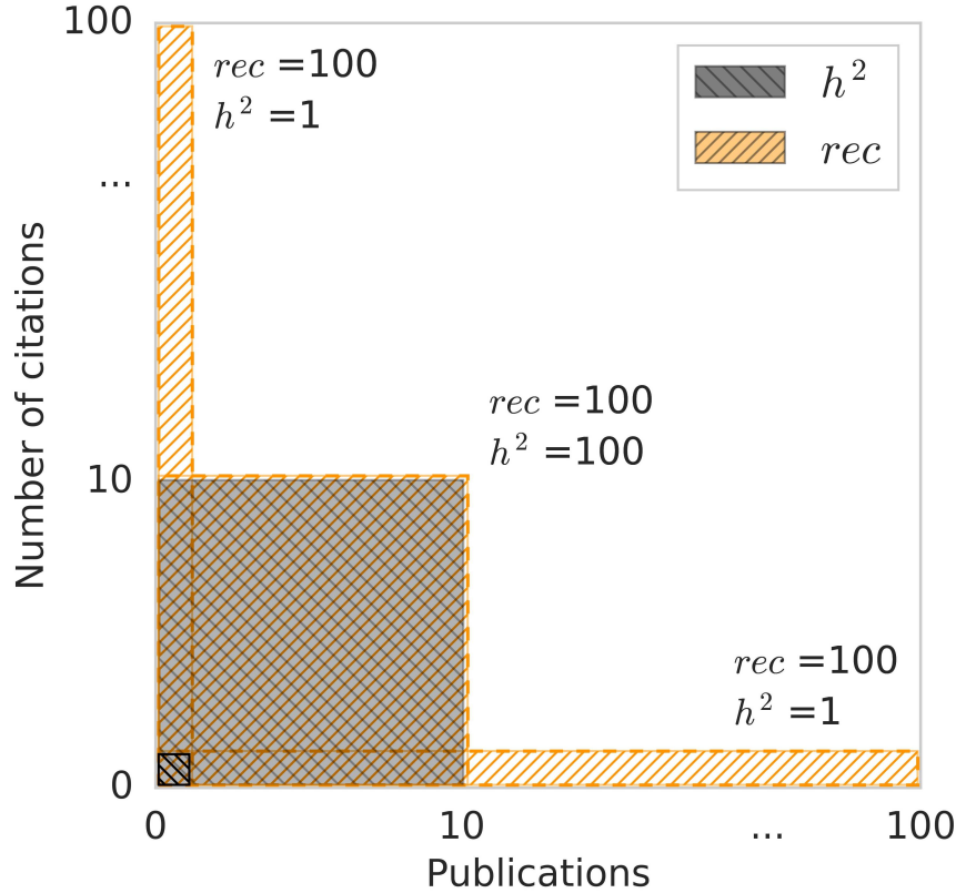
Figure 1: Example of the geometric interpretation of the h^2 and rec indices.
