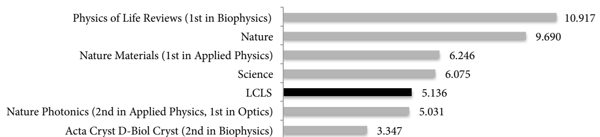
Figure 10: LCLS immediacy index compared to some leading journals in relevant fields (2011)
