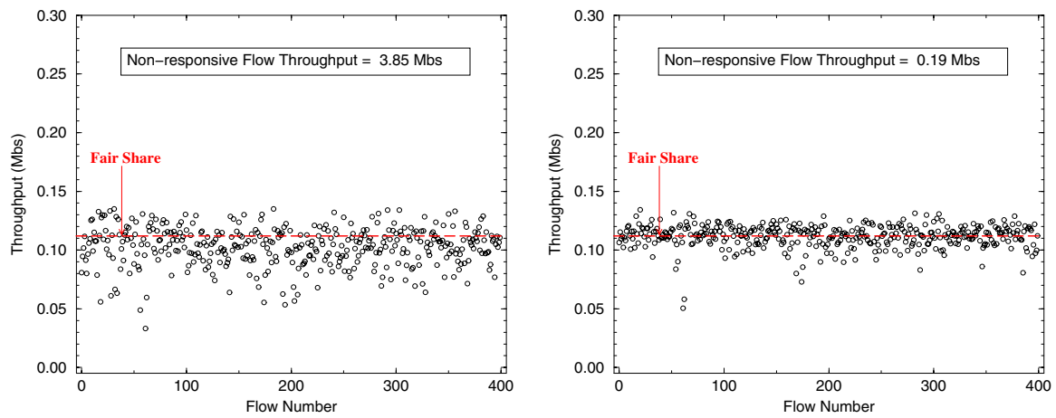
(a) Moving hash (b) Double buffered moving hash Fig. 6. Bandwidth of TCP flows using modified SFB algorithms
