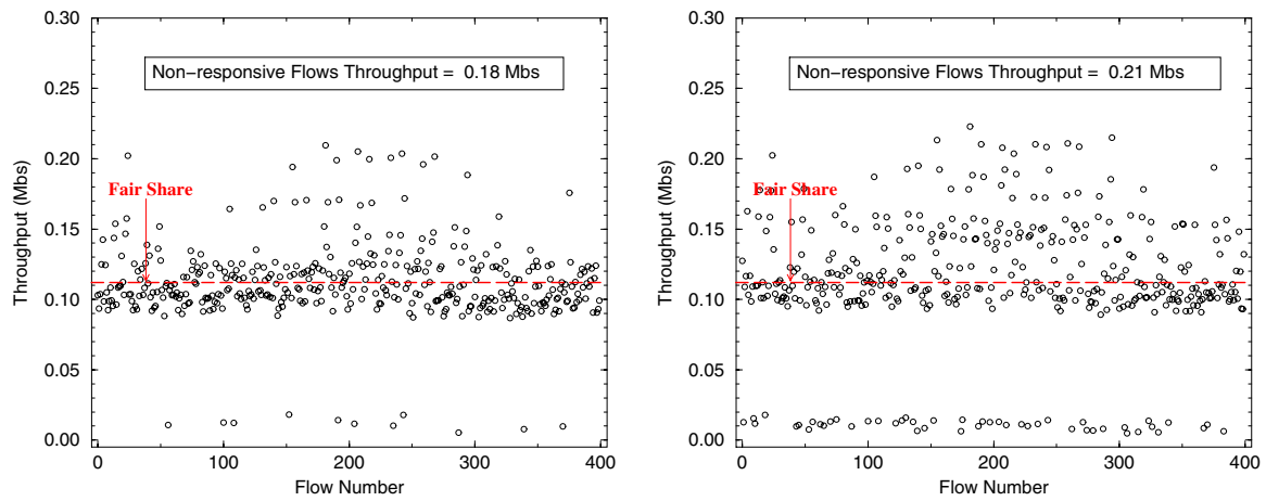
(a) 4 non-responsive flows (b) 8 non-responsive flows Fig. 5. Bandwidth of TCP flows using SFB
