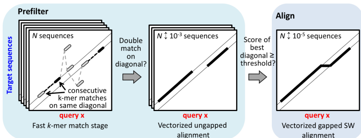
Figure 0.1: Search workflow
