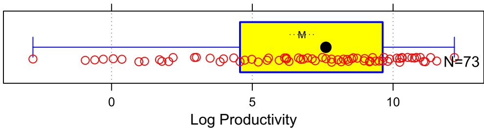
Figure 1-4. “Productivity” for 73 developers for the same small program
