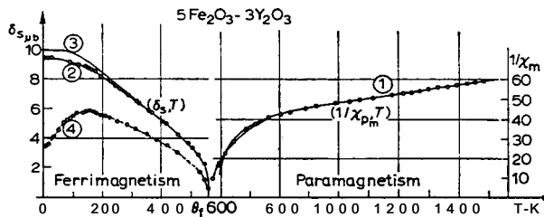
Fig. 20. Yttrium garnet. Temperature dependence of the spontaneous magnetization and of the inverse susceptibility; experimental points and curves calculated using the same molecular field coefficients. Curve (4) refers to a yttrium garnet containing a small amount of gadolinium.
